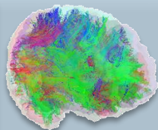
Fiber tracking
