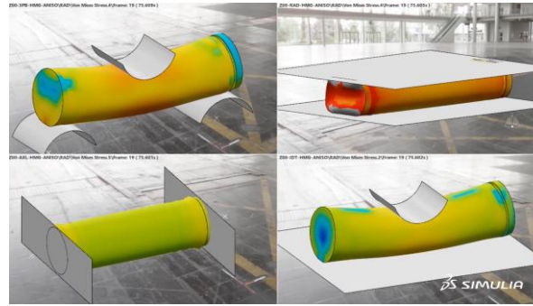
Cell Simulation
