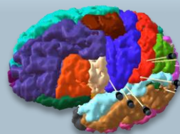
Electrode coregistration
